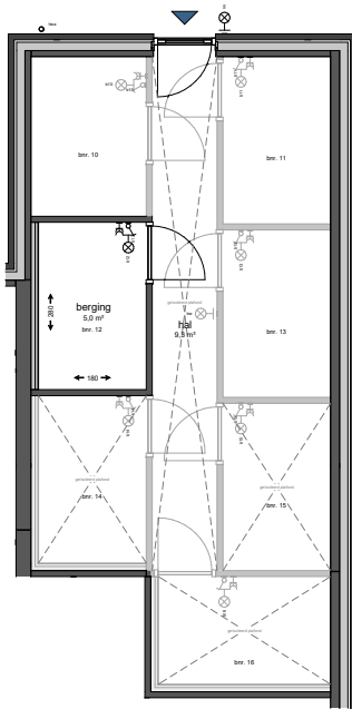
Berging
